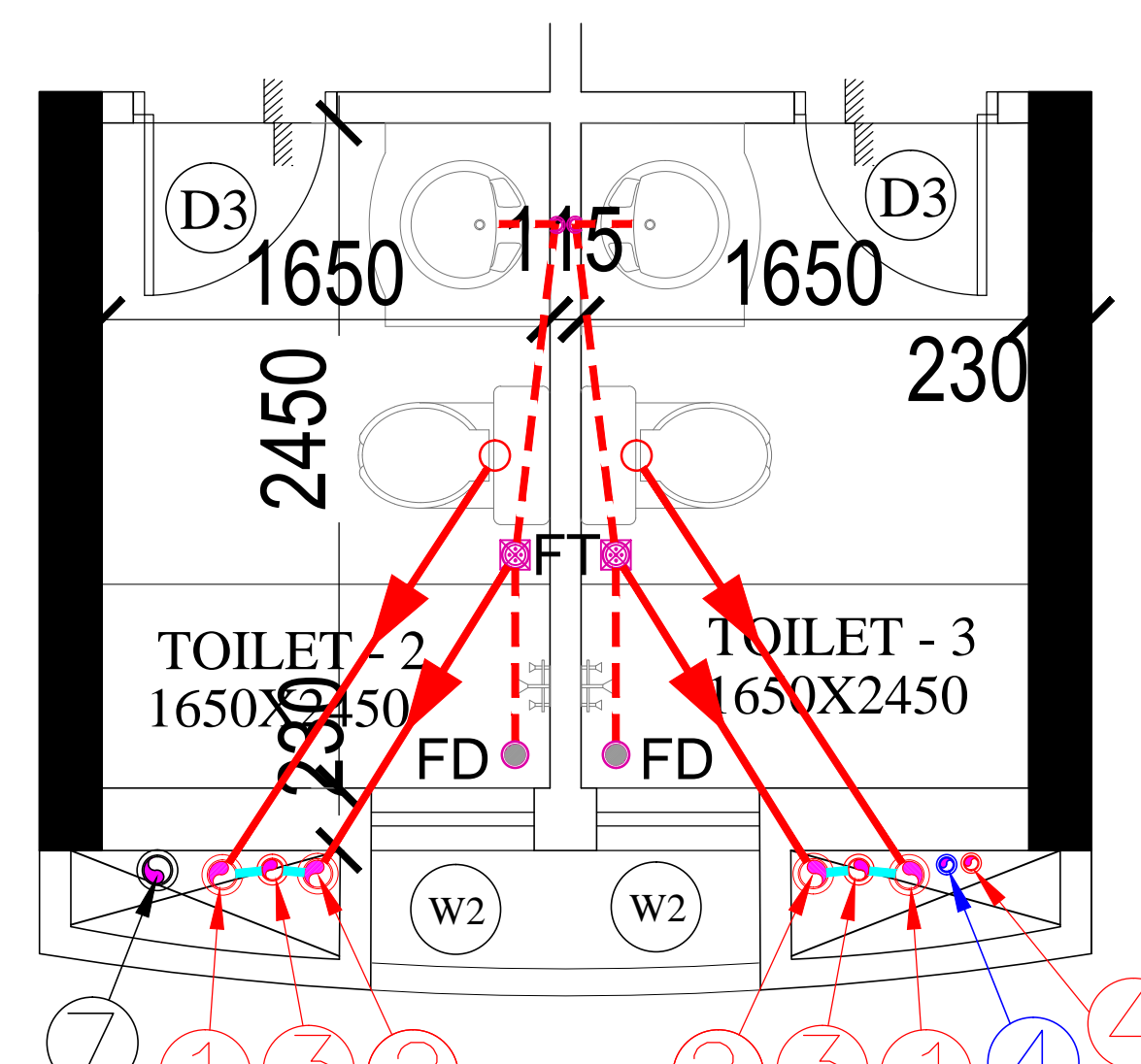
FOURTH FLOOR PLAN FOR TYPICAL TOILET DETAIL (BLOCK - A)
