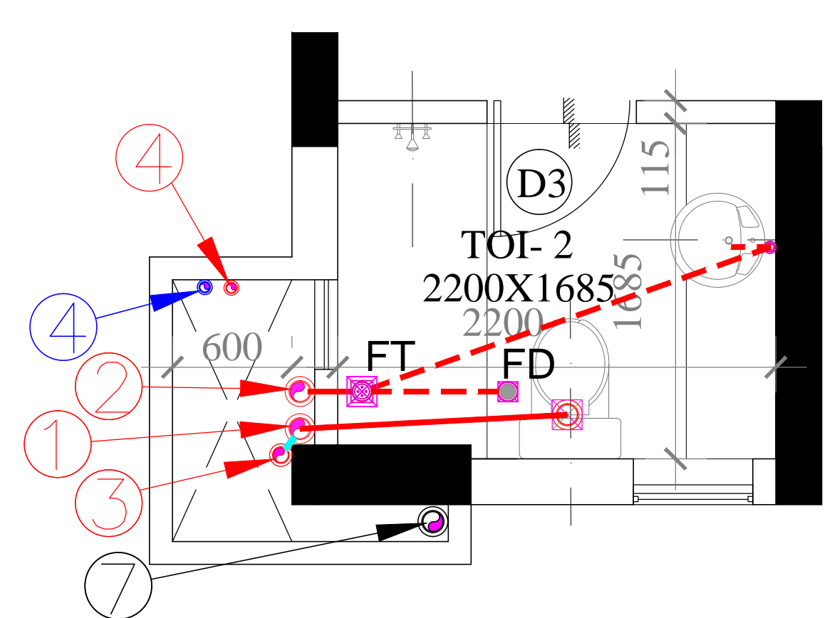
GROUND FLOOR PLAN FOR TYPICAL TOILET DETAIL (BLOCK - B1 & B3)
