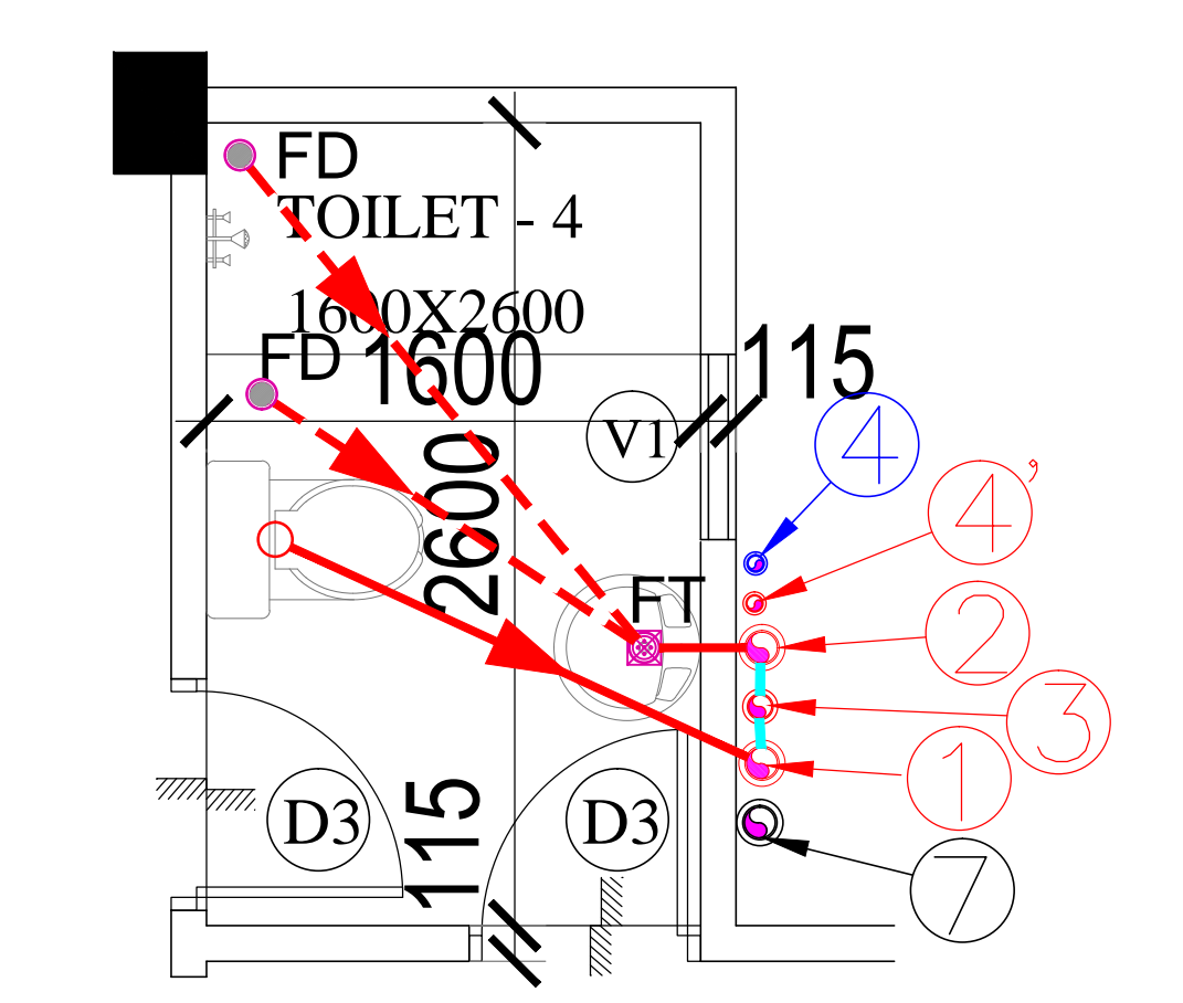
TYPICAL FLOOR PLAN FOR TOILET DETAIL (BLOCK - A)
