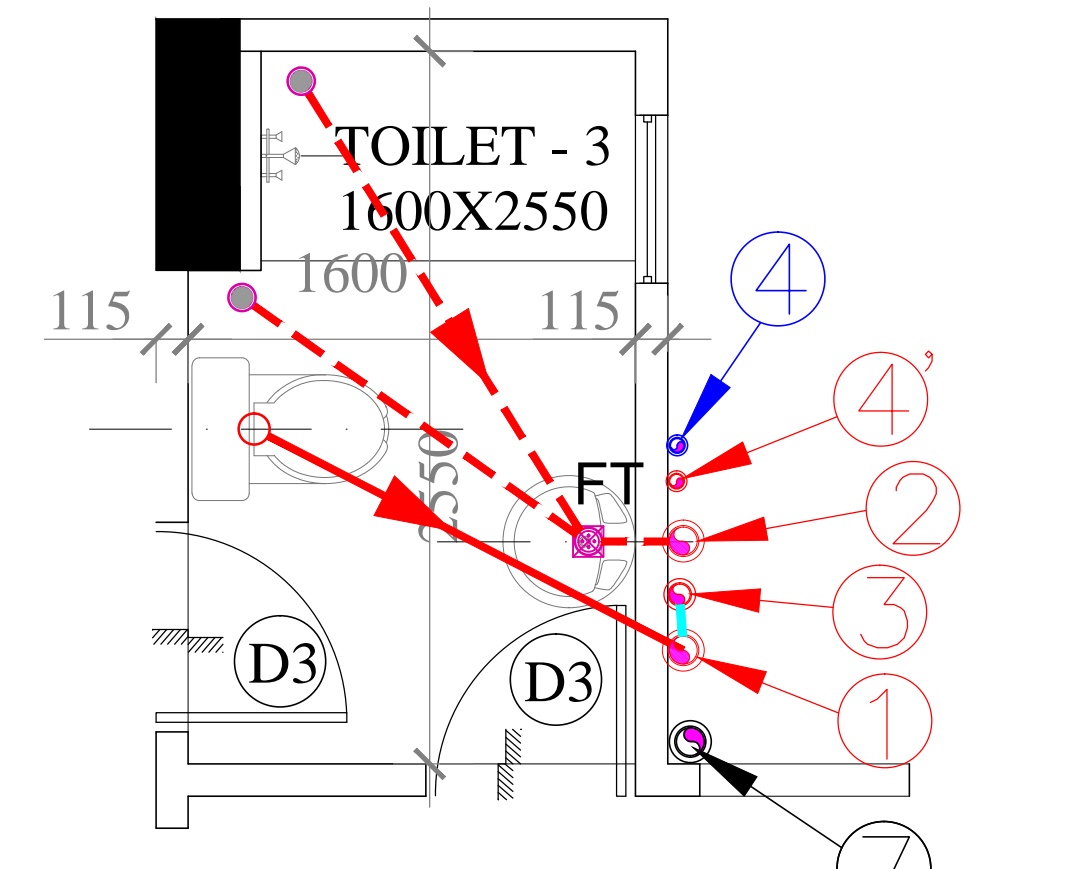
TYPICAL FLOOR PLAN (1ST TO 11TH FLOOR) FOR TOILET DETAIL (BLOCK - B1 & B3)
