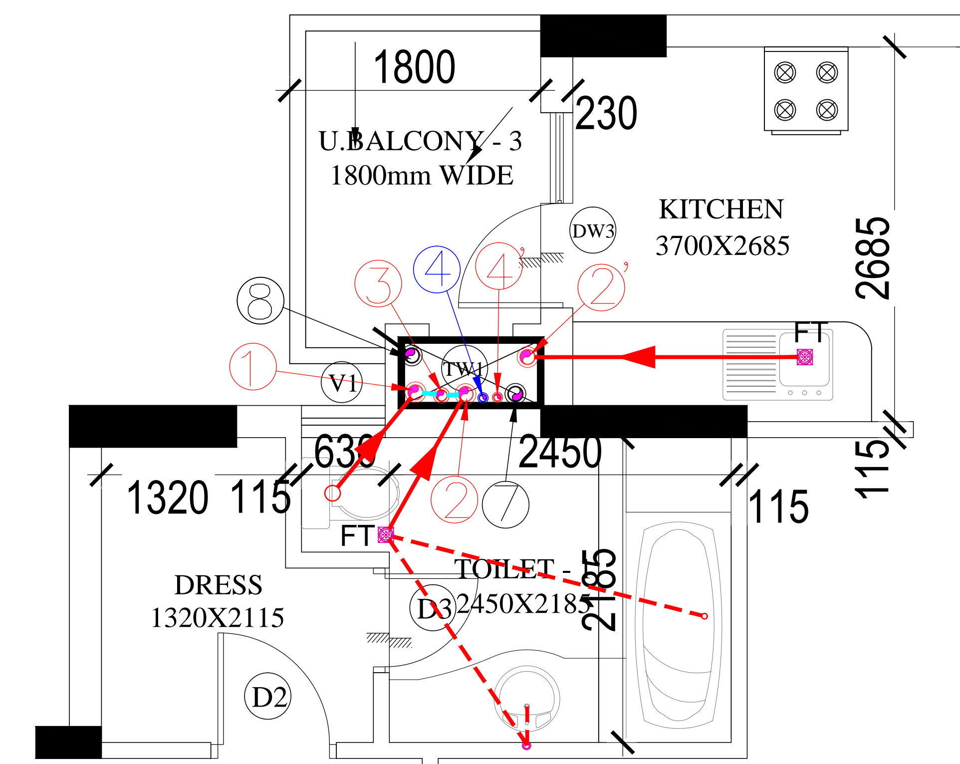
TYPICAL FLOOR PLAN FOR TOILET DETAIL (BLOCK - A)
