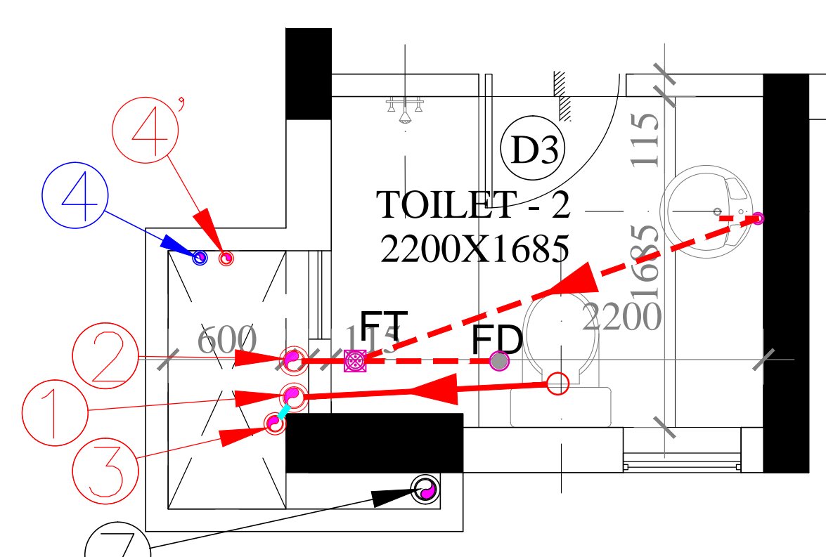
TYPICAL FLOOR PLAN (1ST TO 11TH FLOOR) FOR TOILET DETAIL (BLOCK - B1 & B3)
