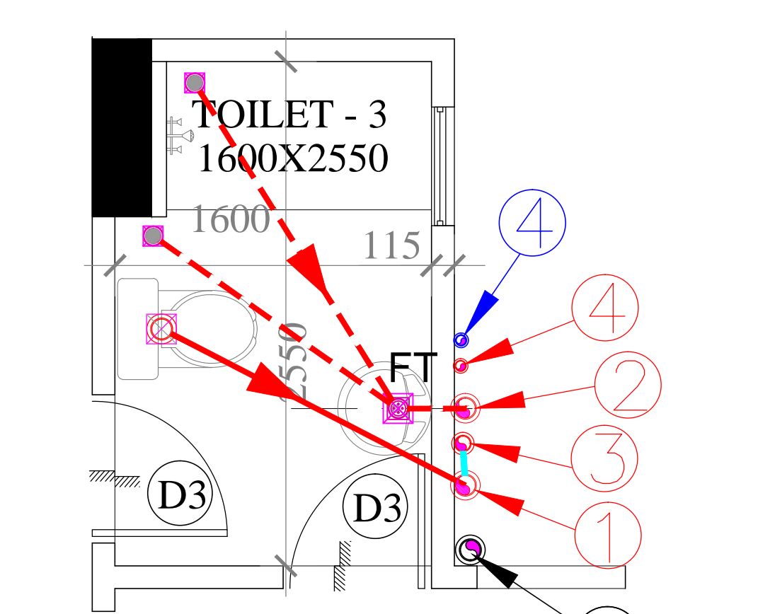
GROUND FLOOR PLAN FOR TYPICAL TOILET DETAIL (BLOCK - B1 & B3)
