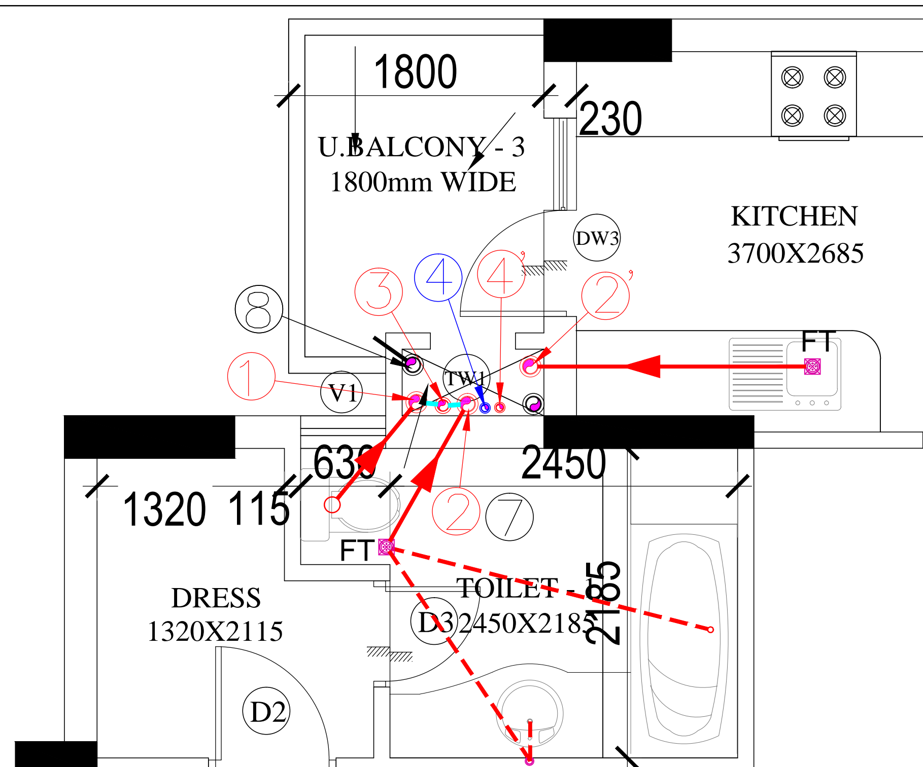
FOURTH FLOOR PLAN FOR TYPICAL TOILET DETAIL (BLOCK - A)
