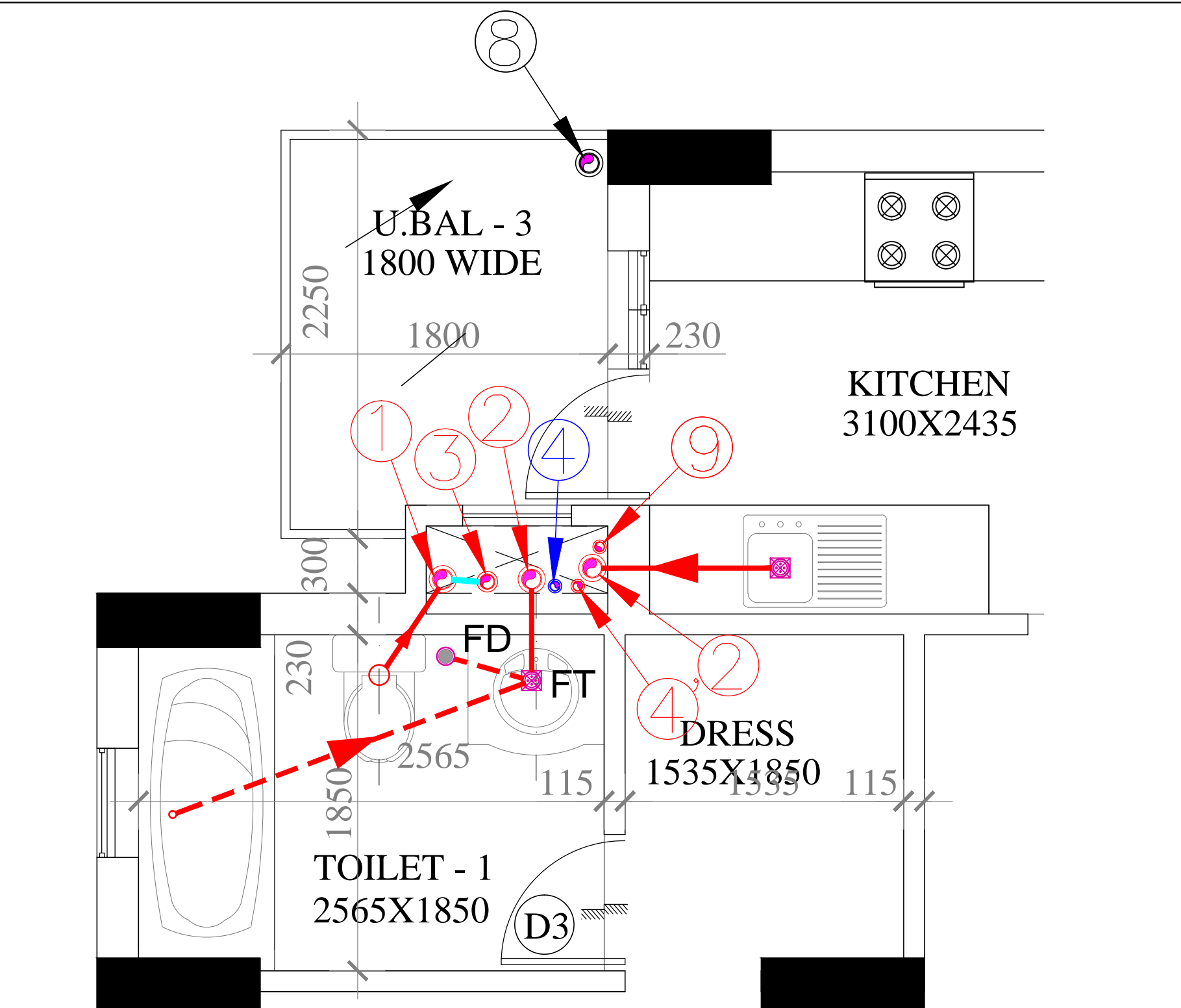
TYPICAL FLOOR PLAN (1ST TO 11TH FLOOR) FOR TOILET DETAIL (BLOCK - B1 & B3)
