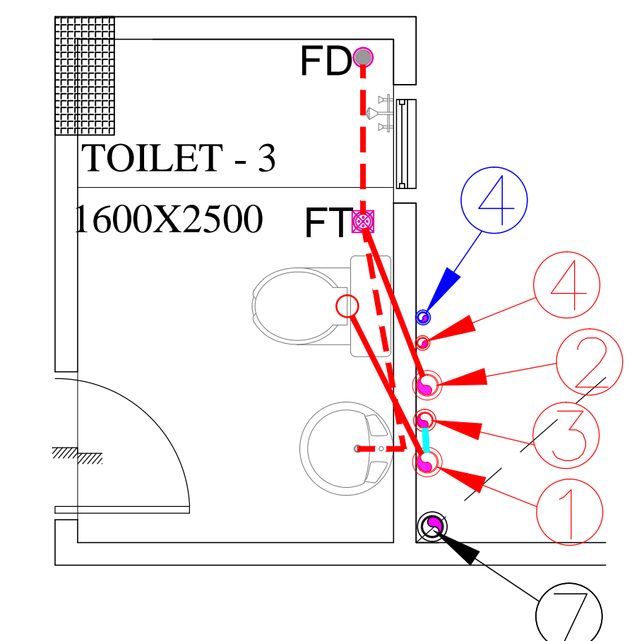
19TH FLOOR PLAN FOR TYPICAL TOILET DETAIL (BLOCK - B1 & B3)
