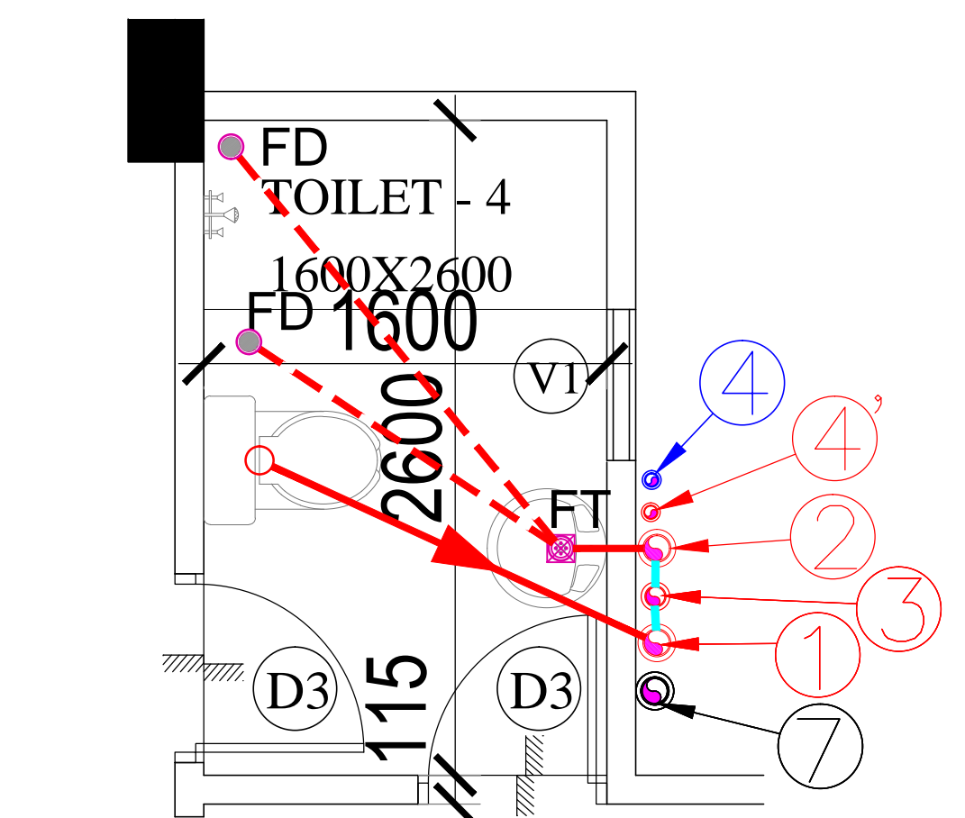
FOURTH FLOOR PLAN FOR TYPICAL TOILET DETAIL (BLOCK - A)
