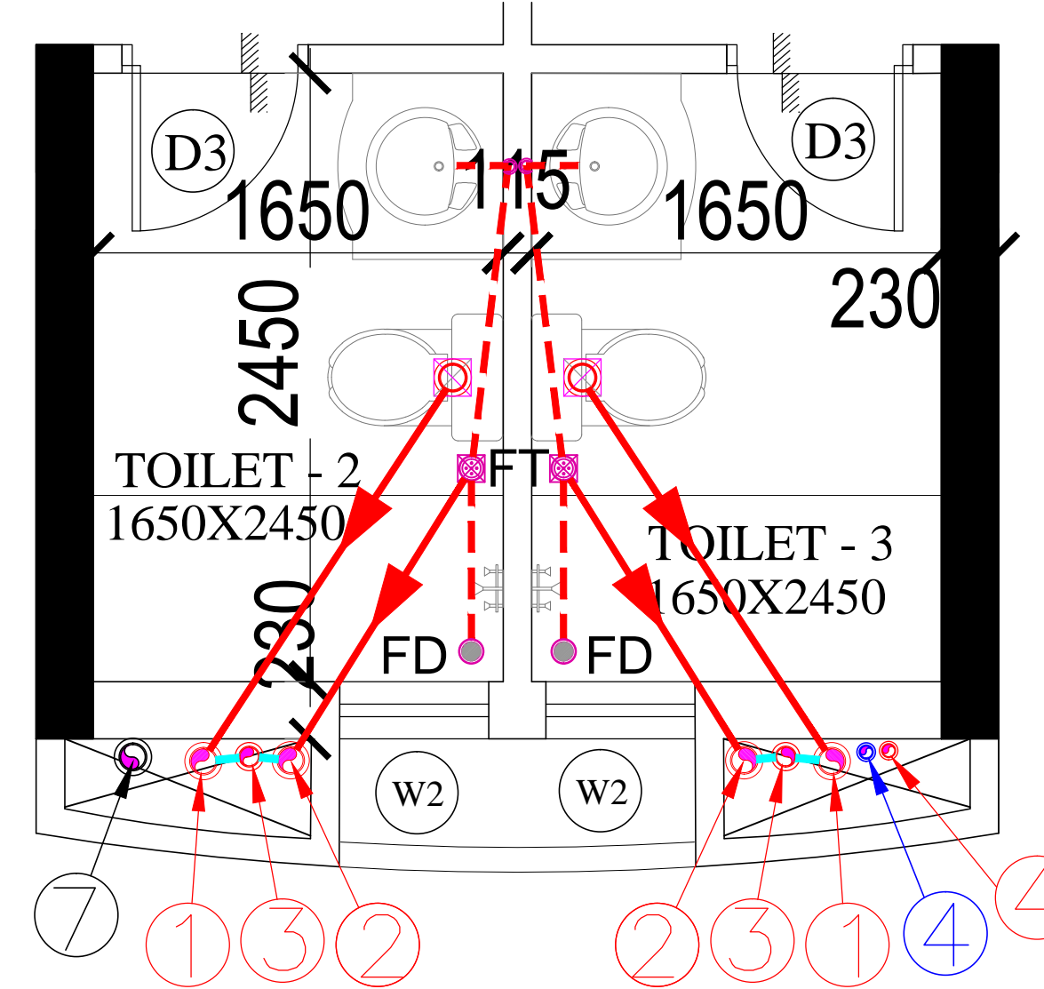
GROUND FLOOR PLAN FOR TYPICAL TOILET DETAIL (BLOCK - A)
