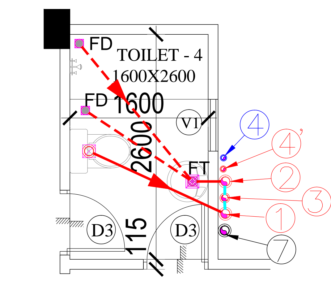
GROUND FLOOR PLAN FOR TYPICAL TOILET DETAIL (BLOCK - A)
