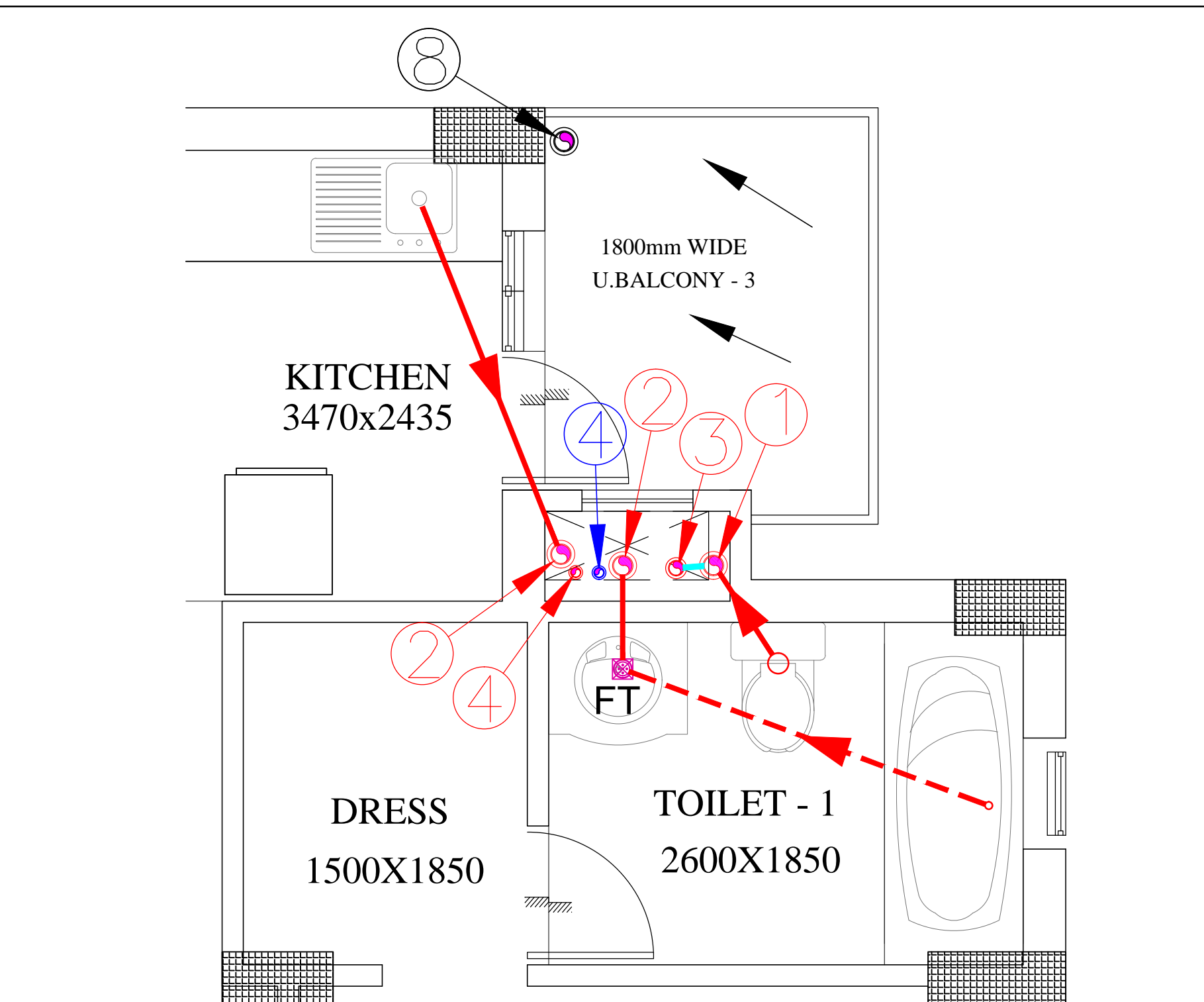
19TH FLOOR PLAN FOR TYPICAL TOILET DETAIL (BLOCK - B1 & B3)
