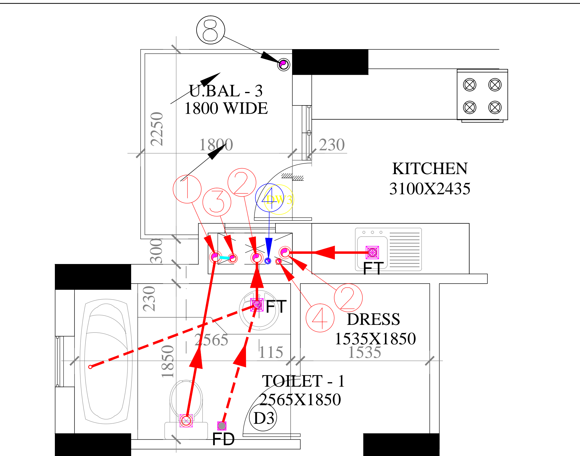
GROUND FLOOR PLAN FOR TYPICAL TOILET DETAIL (BLOCK - B1 & B3)
