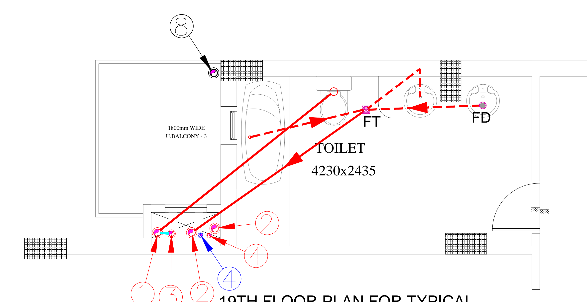
19TH FLOOR PLAN FOR TYPICAL TOILET DETAIL (BLOCK - B1 & B3)
