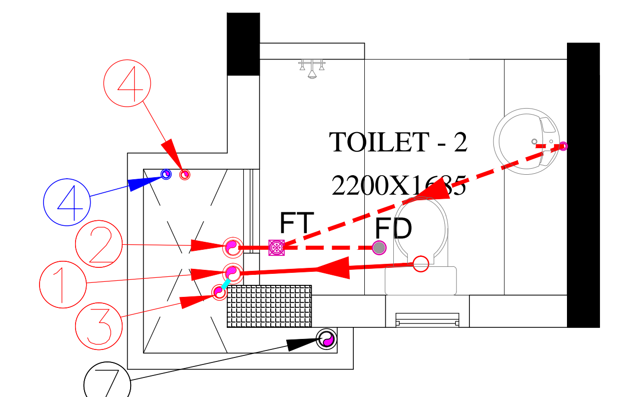
19TH FLOOR PLAN FOR TYPICAL TOILET DETAIL (BLOCK - B1 & B3)
