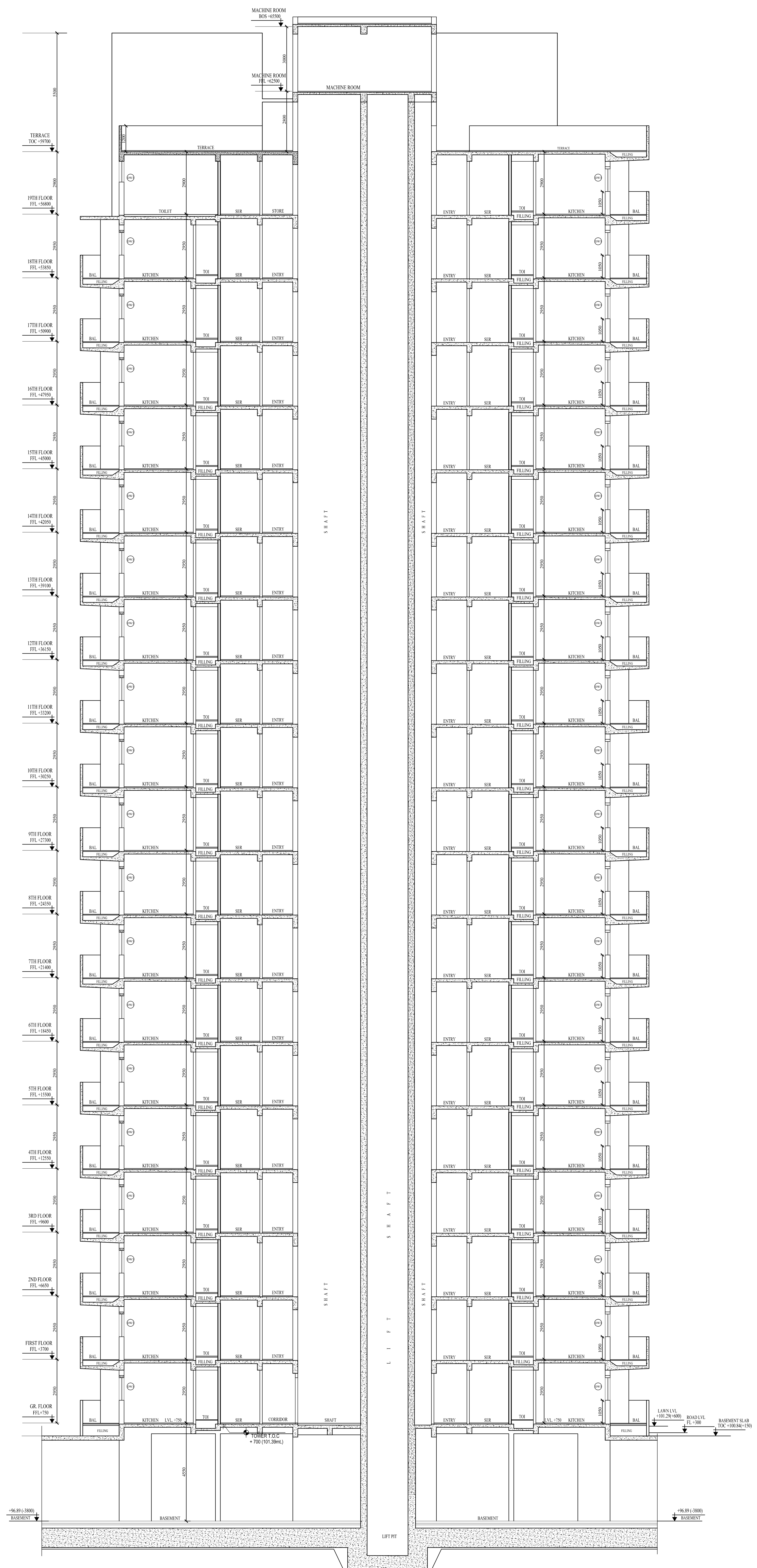
SECTION AT 02
